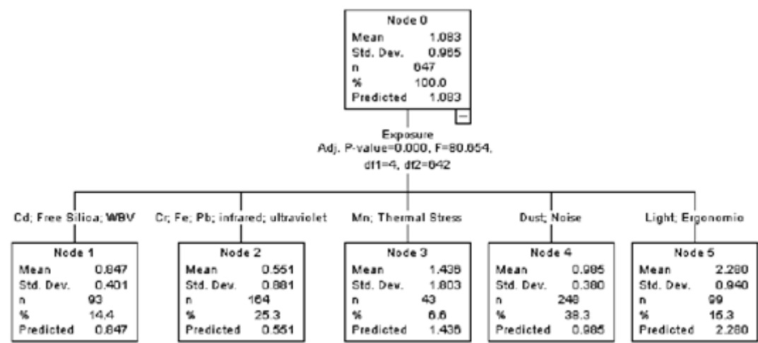
Fig. 1. CHAID Output Classified diagram of ESR Variable
